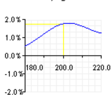
Rho/ Underlying
