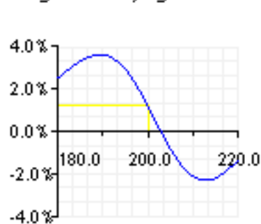
Vega/ Underlying
