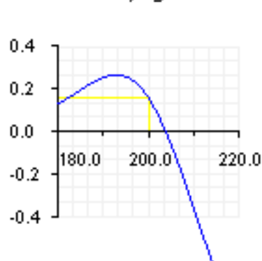
Vega/ Underlying
