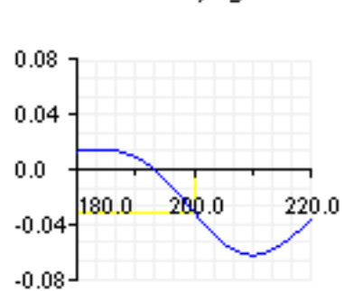
Gamma/ Underlying
