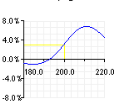
Theta/ Underlying
