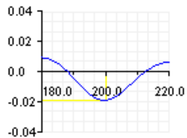
Gamma/ Underlying
