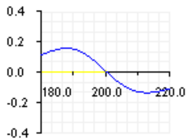
Delta/ Underlying
