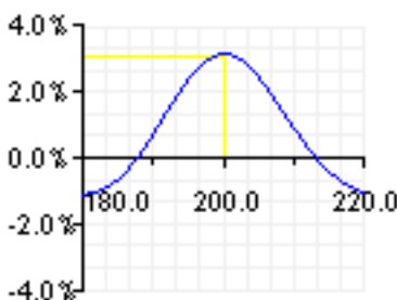
Theta/ Underlying
