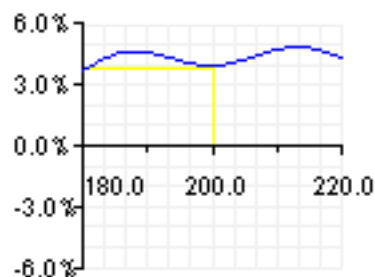
Vega/ Underlying
