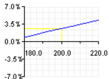
Rho/ Underlying
